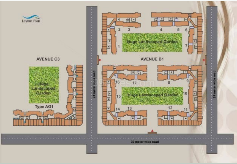
Master Plan
